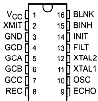
N PACKAGE (TOP VIEW)
