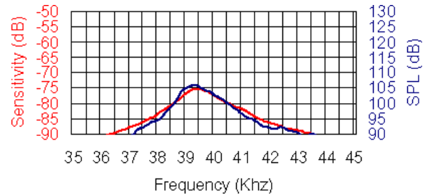
Sensitivity/Sound Pressure Level Tested under 10 Vrms @ 30 cm
