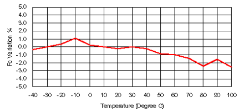
Transmitter Center Frequency Shift vs. Temperature
