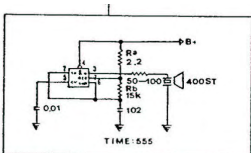
SUGGESTED OSCILLATING CIRCUITS
