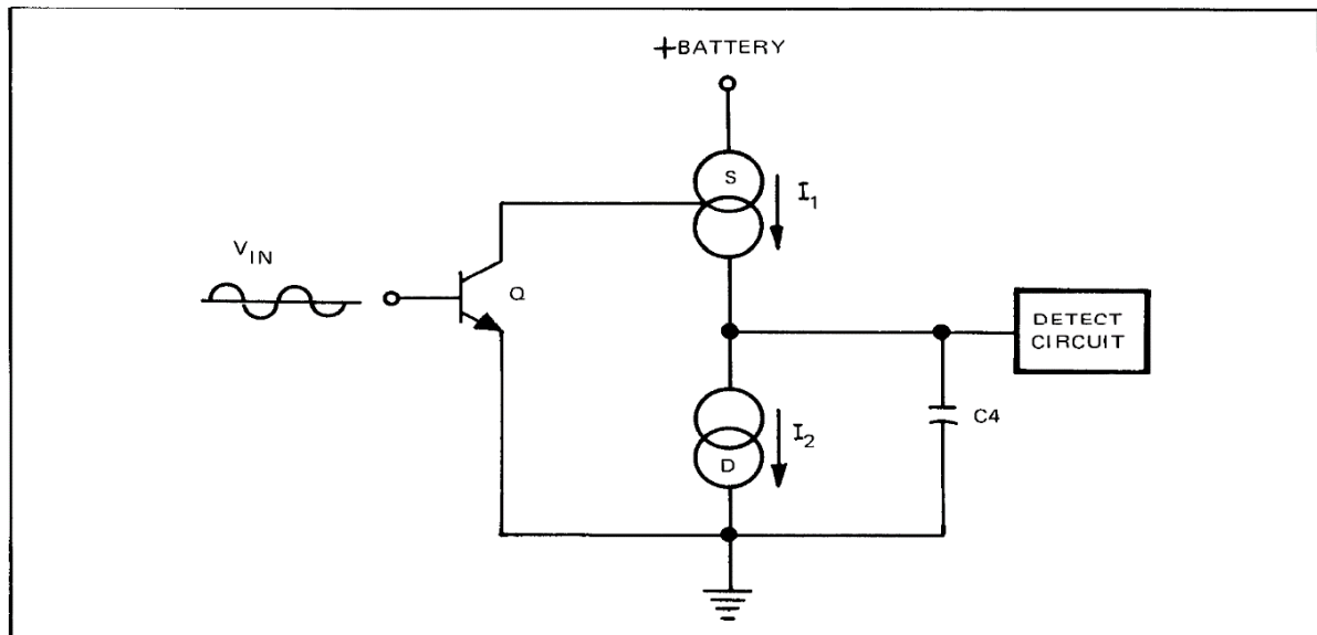
FIGURE 4-12 DETECTION CIRCUIT
