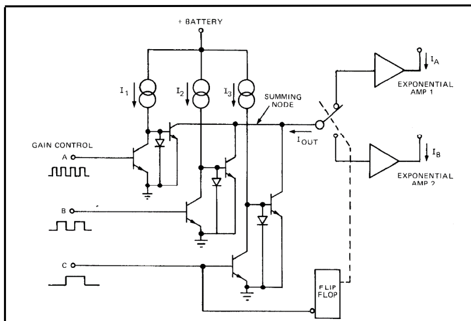
FIGURE 4-17 D / A CONVERTER
