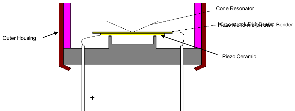
FIGURE 4-8 PIEZOELECTRIC TRANSDUCER
