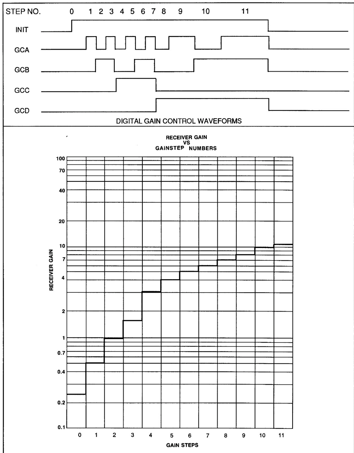
FIGURE 4-18 GAIN CONTROL
