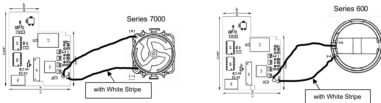
Figure 2-1 Electrostatic Connections
