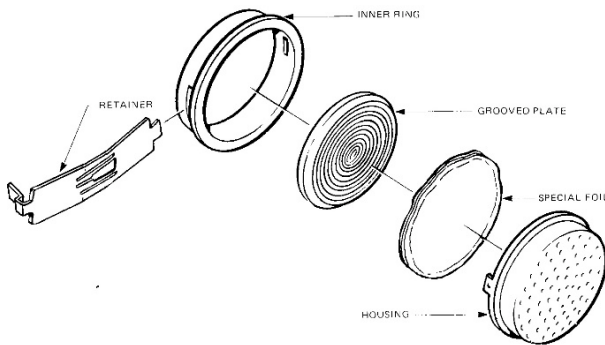
FIGURE 1-1 SERIES 600 TRANSDUCER
