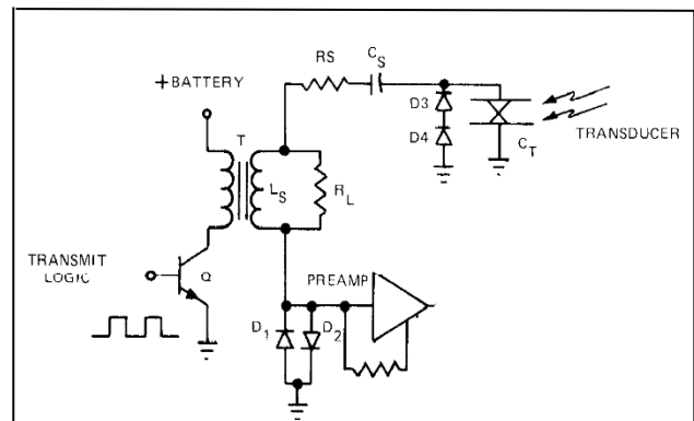
FIGURE 4-9 TRANSMIT CIRCUIT
