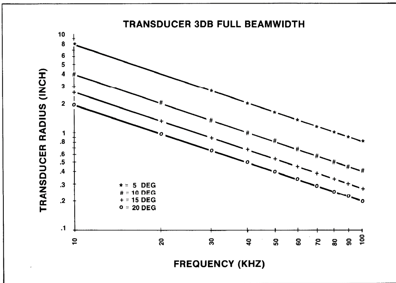
Figure 4-1 BEAMWIDTH / FREQUENCY / RADIUS
