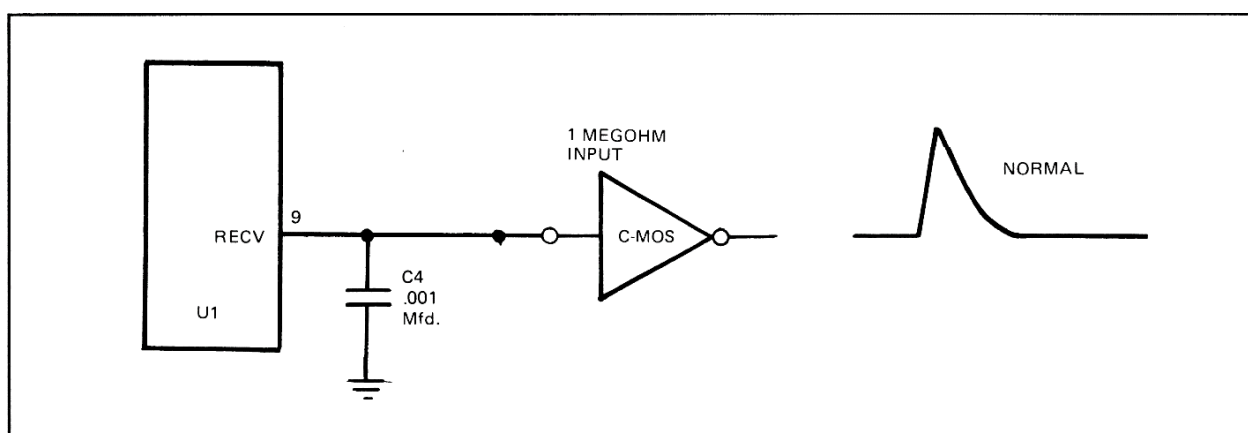
FIGURE 3-6 MODIFIED ECHO DETECTOR
