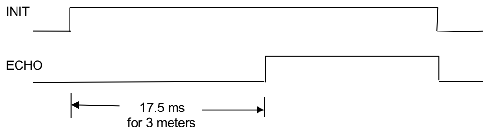
Figure 2-4 – INIT/ECHO Timing
