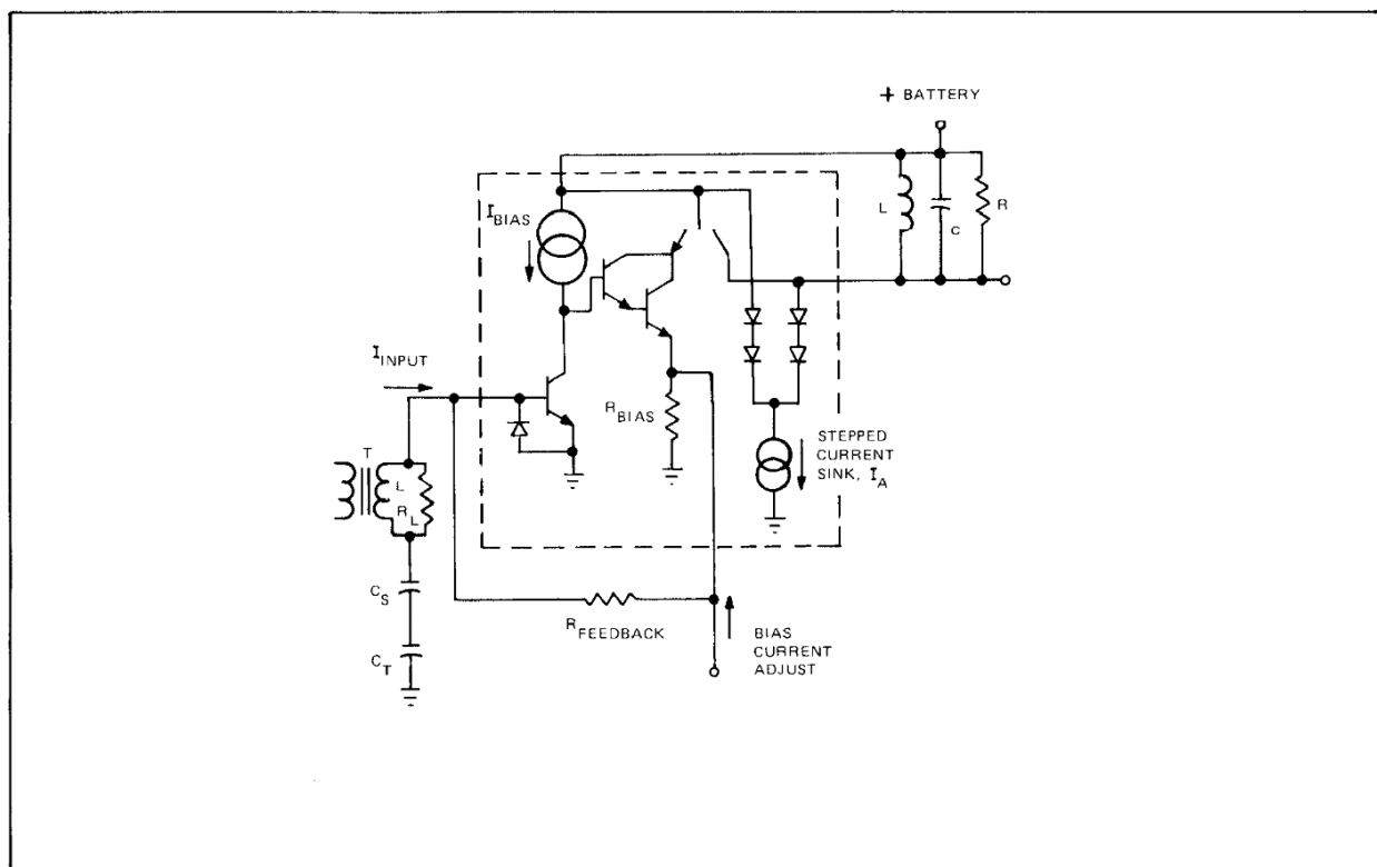
FIGURE 4-11 PREAMPLIFIER CIRCUIT
