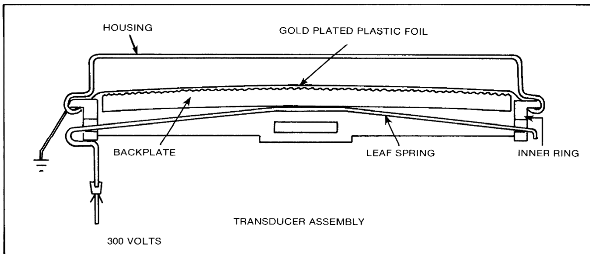
Figure 4-4 Electrostatic Transducer
