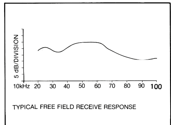
FIGURE 4-6 RECEIVE RESPONSE
