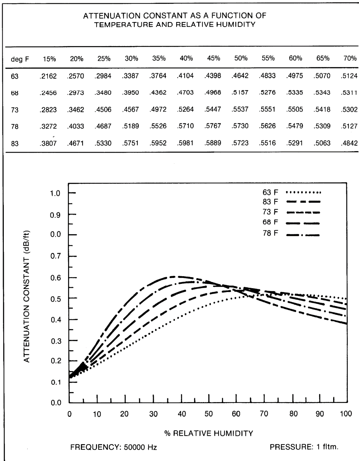
FIGURE 4-3 ATTENUATION CONSTANT
