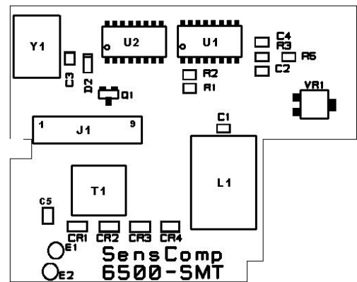
FIGURE 1-2 RANGING MODULE
